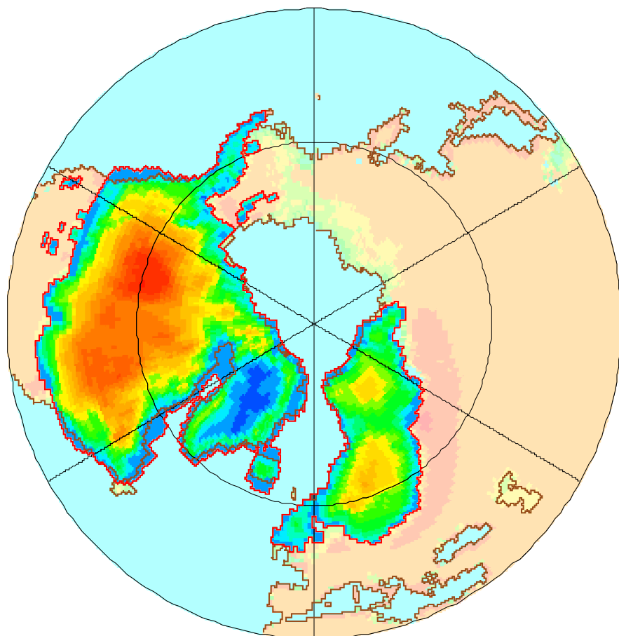
PMIP3 LGM Ice Sheet Masks & Altitude DIFFERENCE (m) 21ka - 0ka
